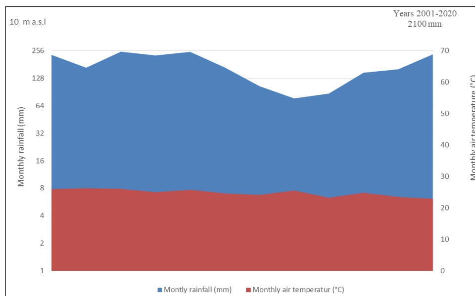
Fig 2: Graph Monthly Rainfall (mm) and Air Temperature (° C) Monthly Year 2001-2020
